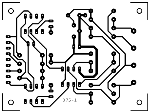
"Opentherm" monitor
