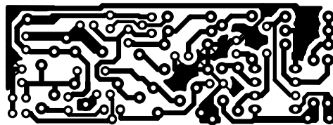
Car alarm 628 - Rx
