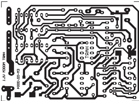
HART modem
